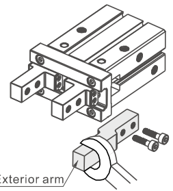
Exterior arm
