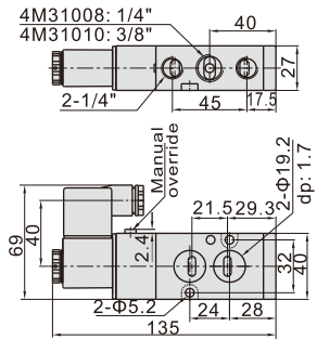
4M310(Terminal)
