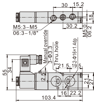
4M110(Terminal)
